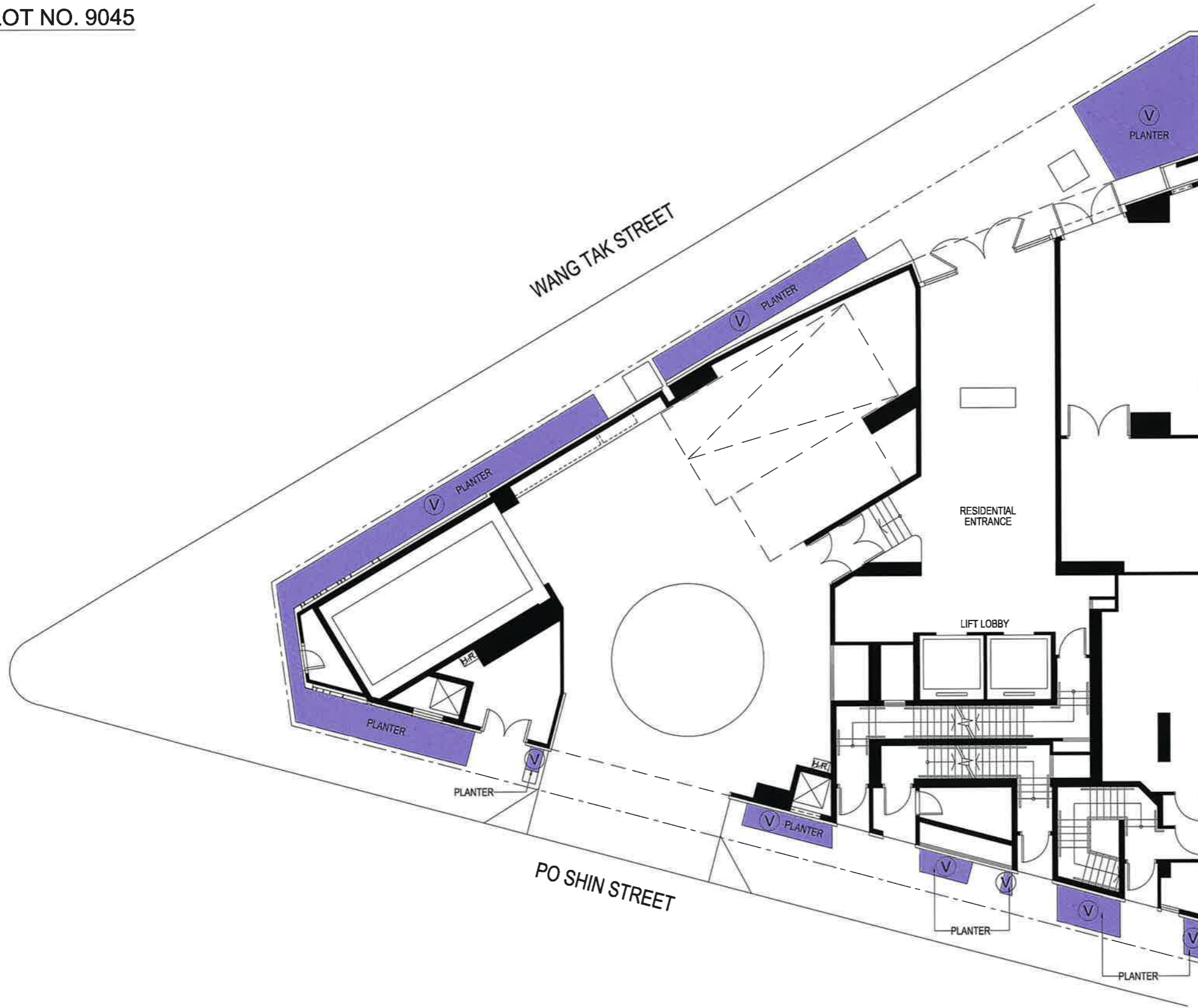
G/F GREENERY AREAS LAYOUT PLAN SCALE : N.T.S.
